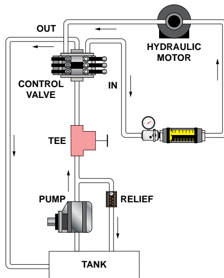
Figure 7: Tee test
